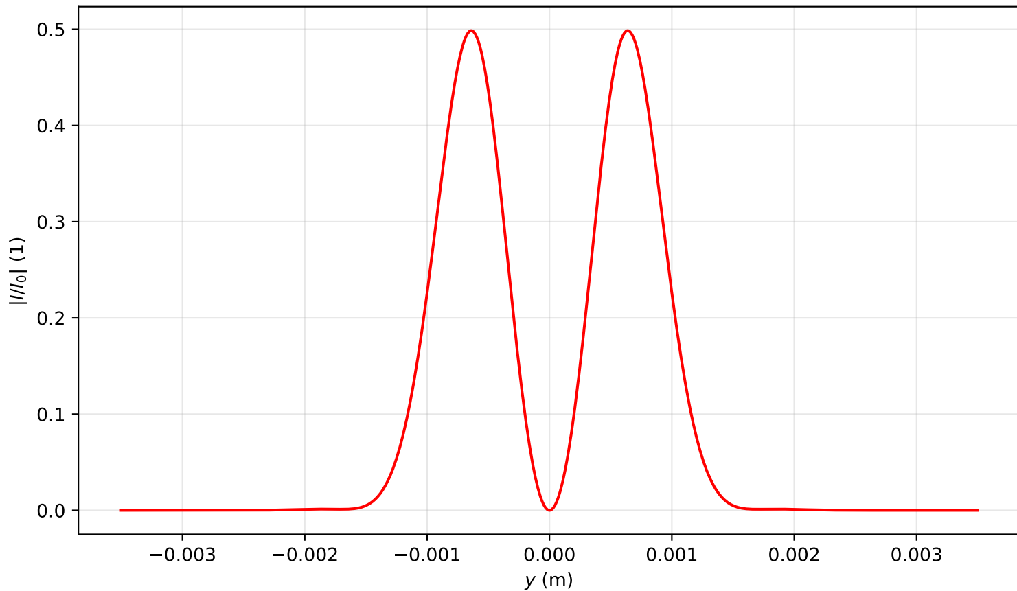
Intensity profile I(x=0, y, z=1.592)/I_0 , P_{in}=2.0P_{cr} , artificial time
